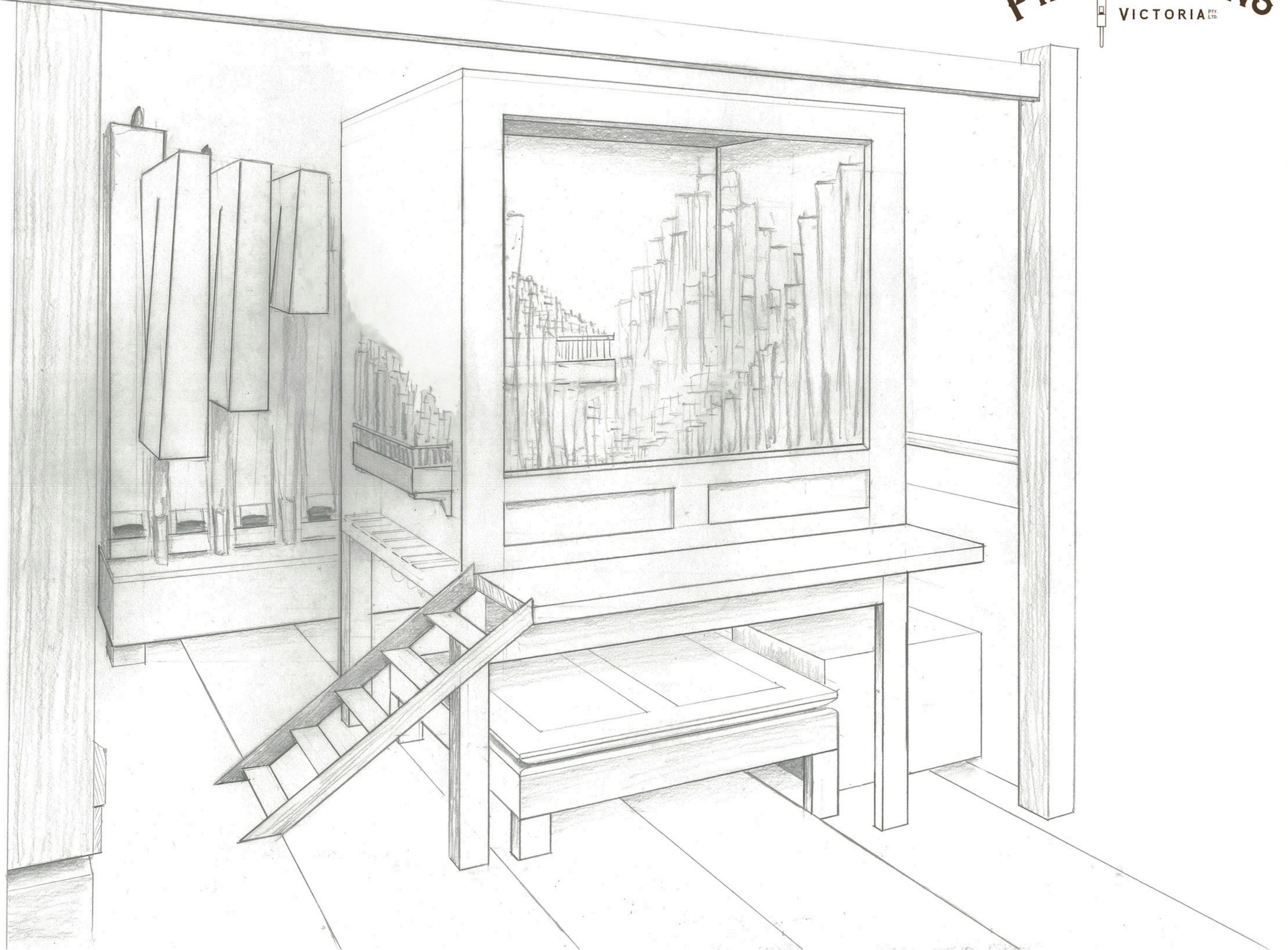
Swell Organ and Pedal C# Side - Internal View (not to scale)
