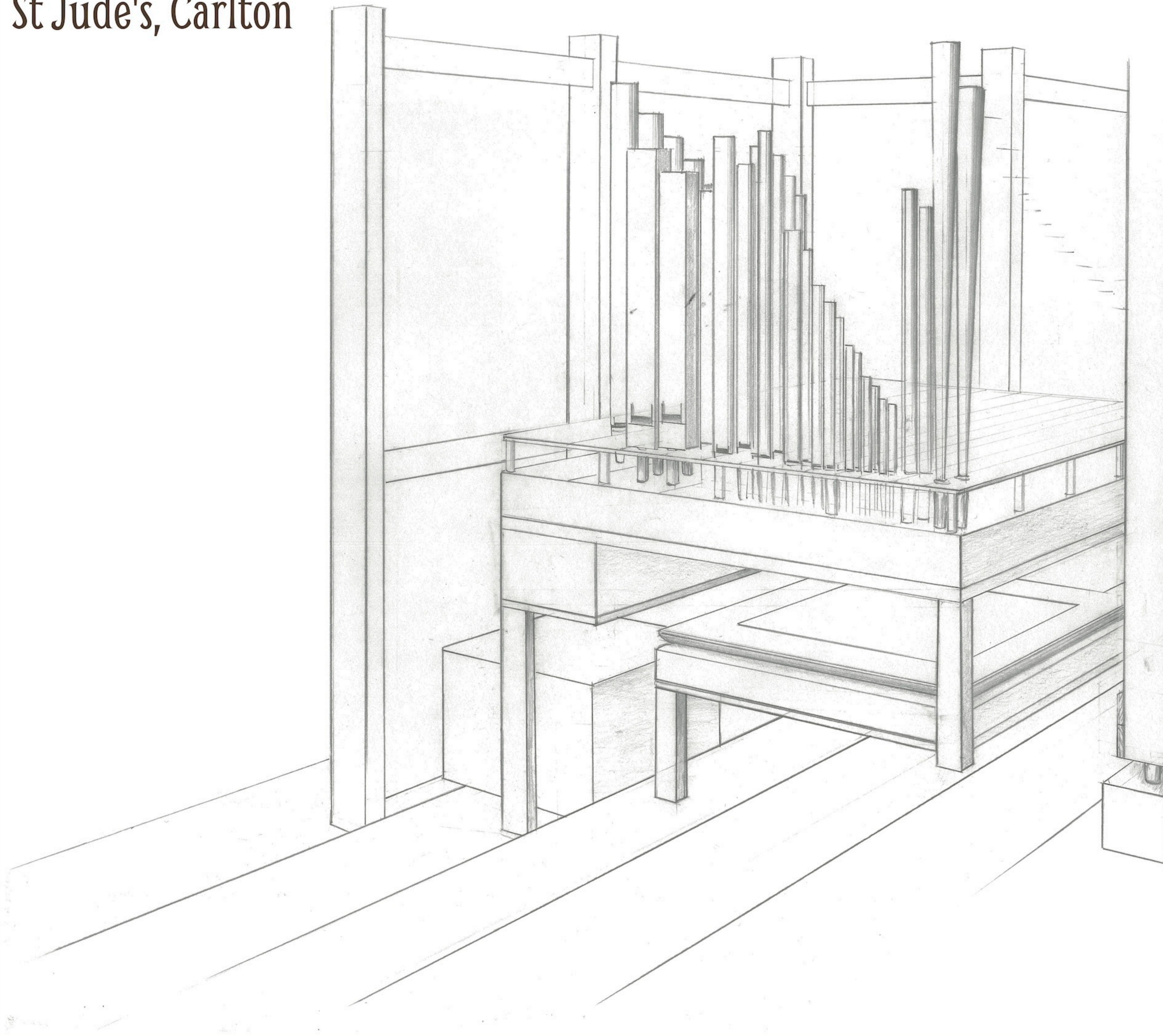
Great Organ and Pedal C Side - Internal View (not to scale)
