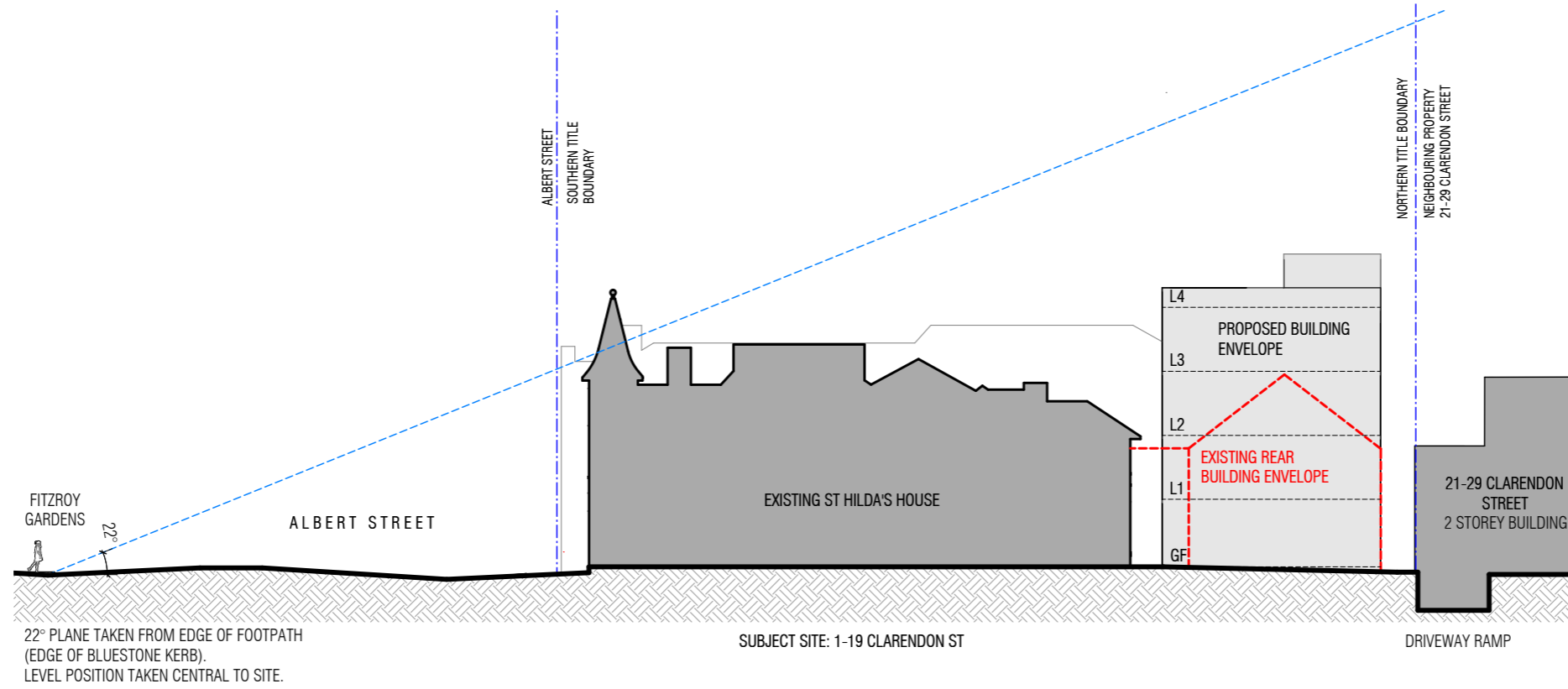
Proposed Building Envelope
