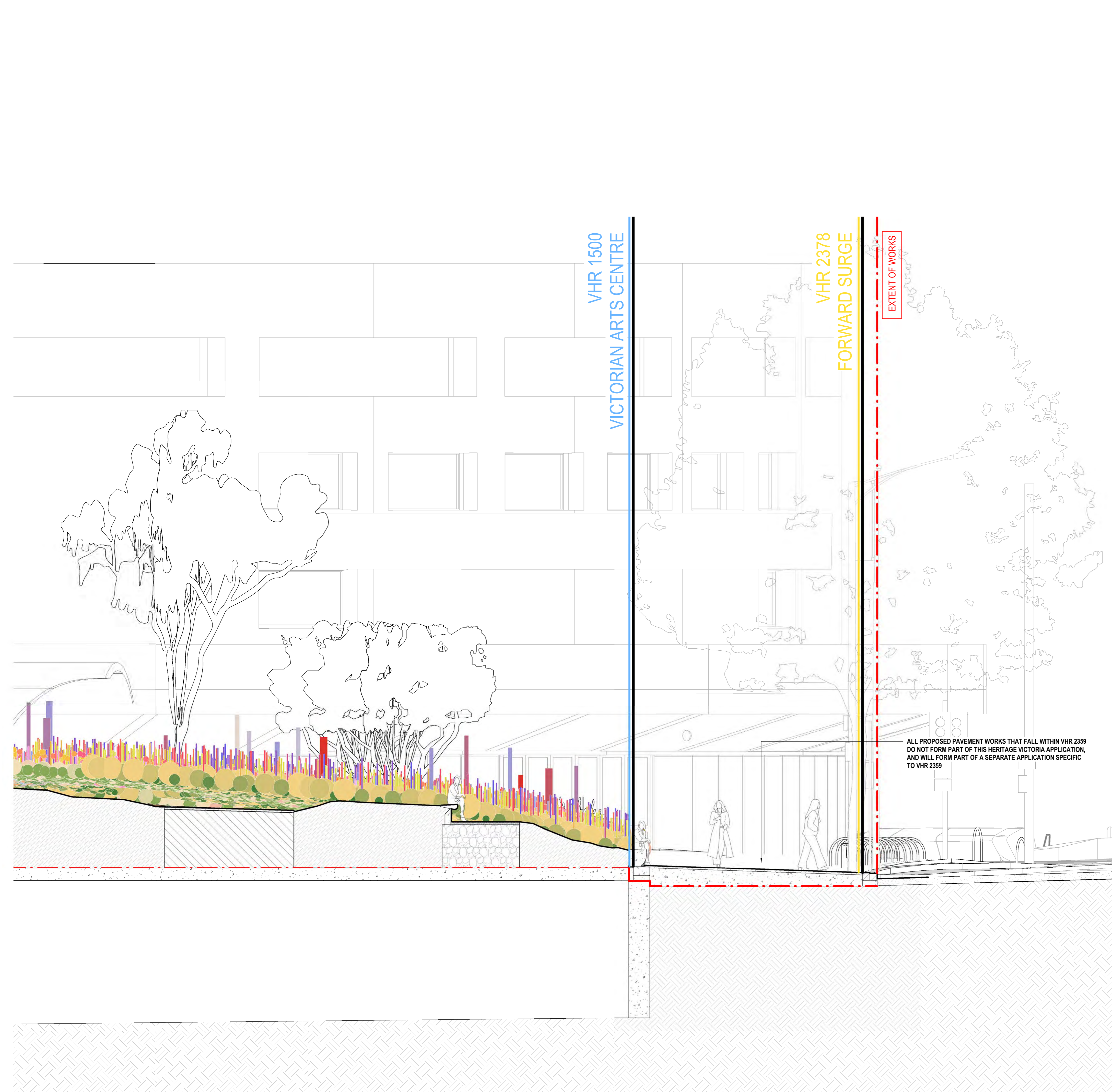
1 INTERFACE SECTION 04 1:50
