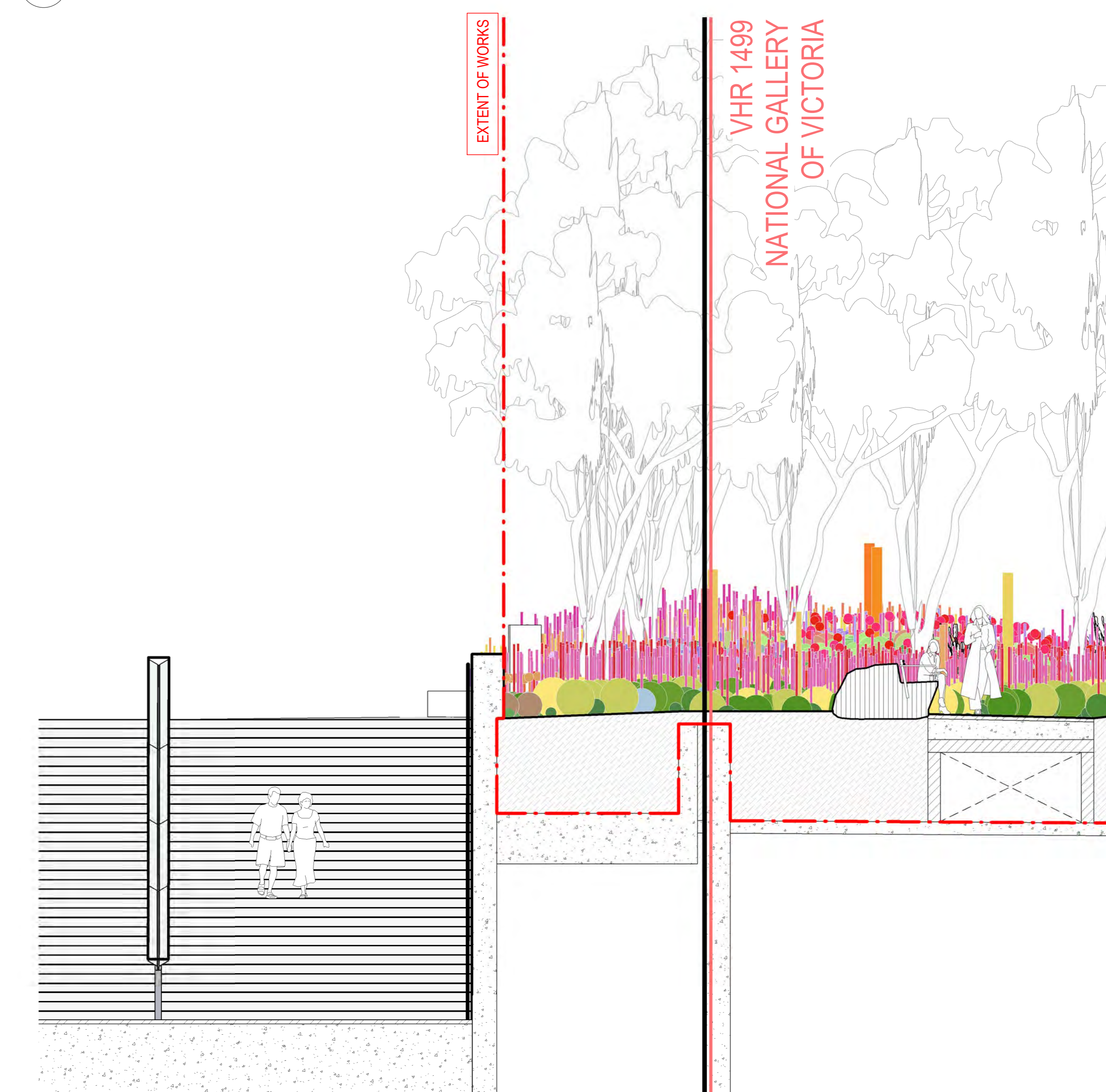
3 INTERFACE SECTION 06 1:50
